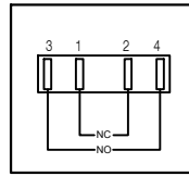
Switching Circuit
